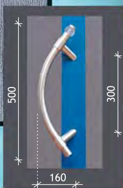
ART. 28.300.21.R.PK MAT. INOX \varnothing 28
