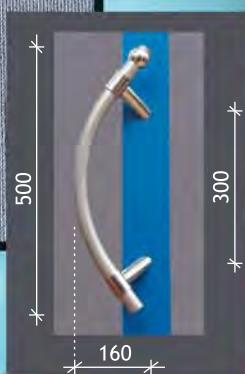
ART. 28.300.21.R.IK MAT. INOX \varnothing 28
